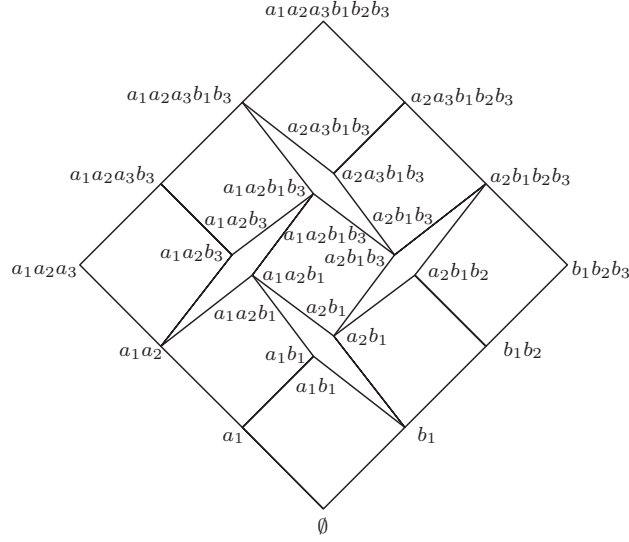
Figure 3: An counter-example which is not \sigma -decomposable
