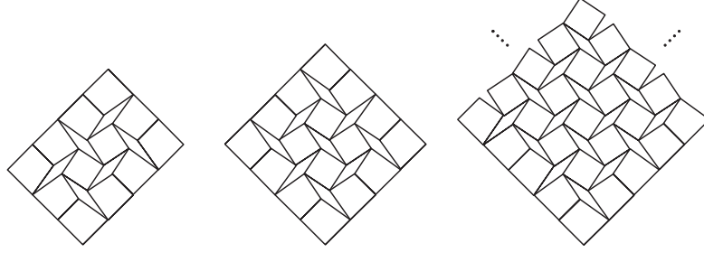
Figure 5: \sigma -indecomposable rift patterns
